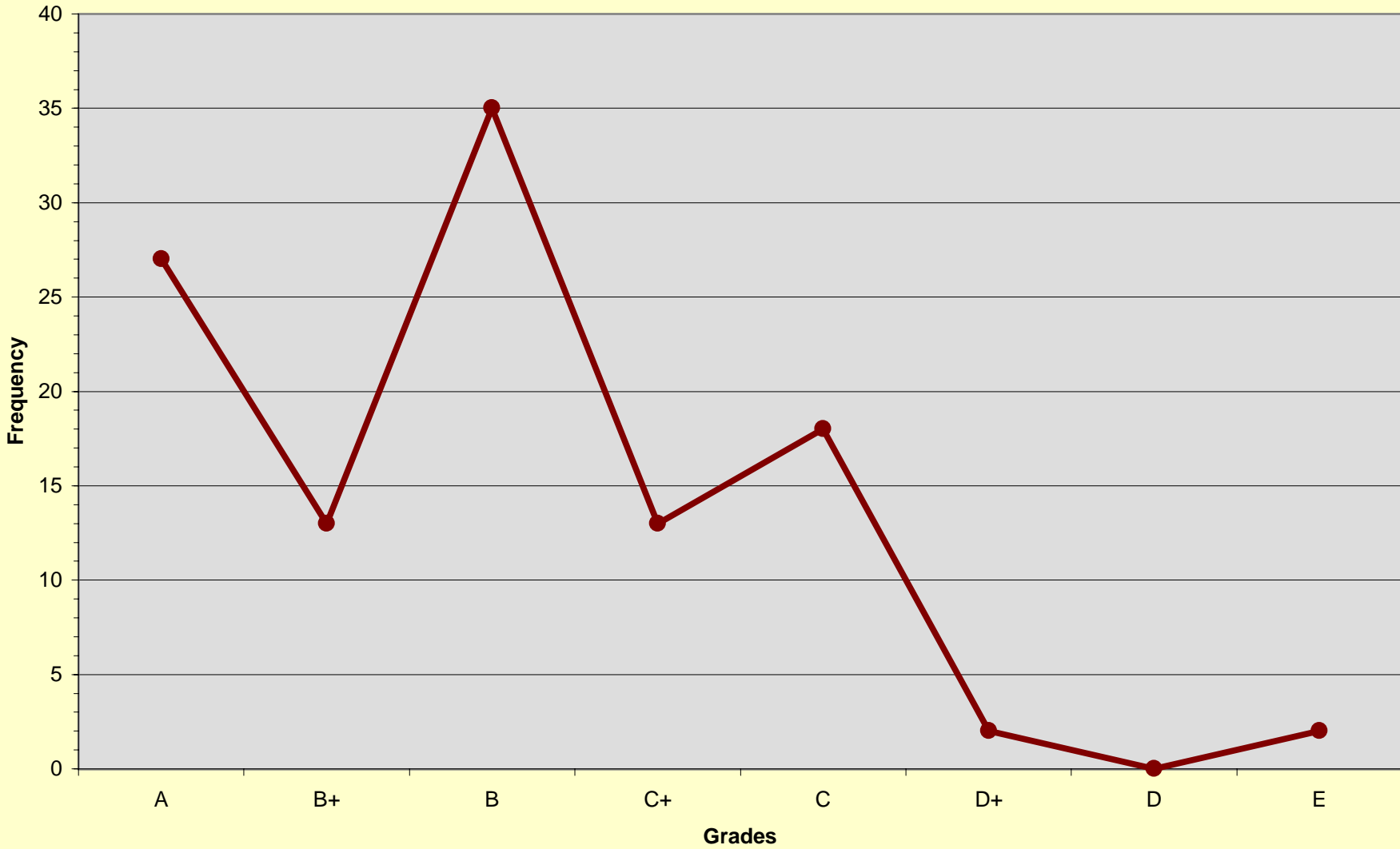
Grade Frequency Distribution
